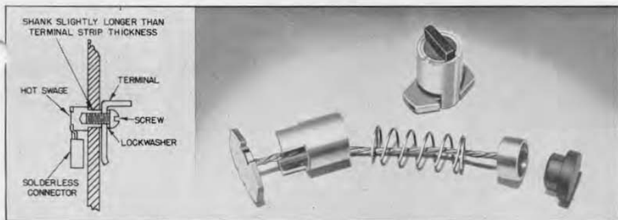
FIGURE 8. Sectional drawing of terminal assembly.
