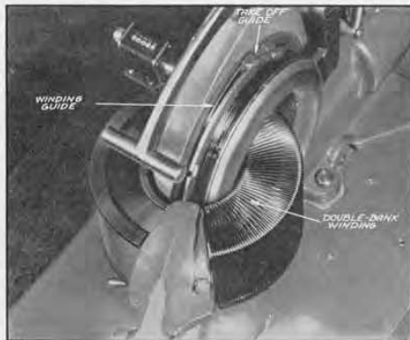
(Below) FIGURE 4. A partially wound V-10 coil.
