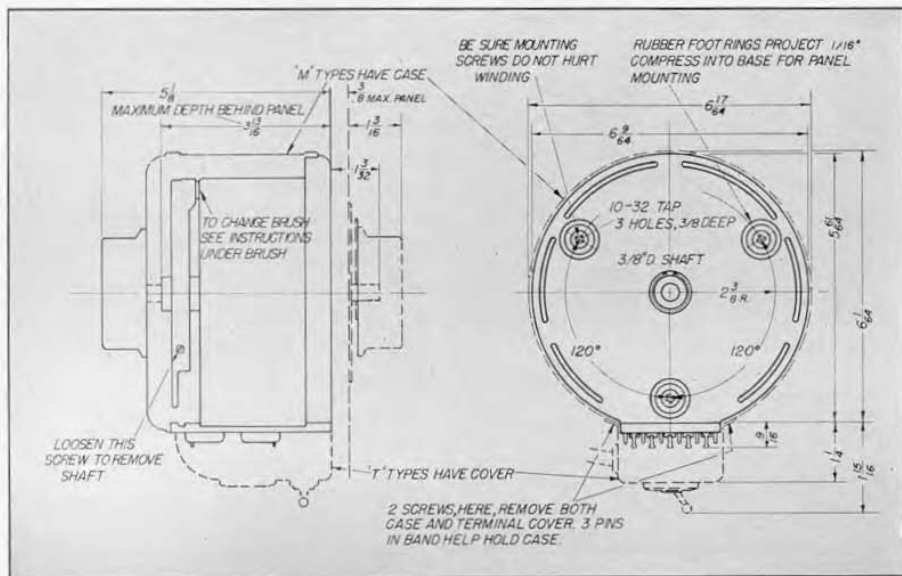
FIGURE 10. Universal dimension sketch for V-10 series Variacs.
