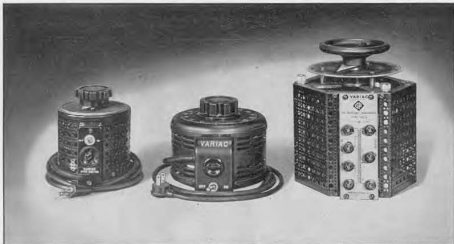
FIGURE 1. Intermediate between the old TYPE 200-CM (left) and the TYPE 100-A (right), the new TYPE V-10 Variac is rated at 10 amperes for 115-volt input.
