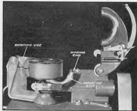
FIGURE 2. Core and winding plate assembly are inserted with winding head assembly opened. Note particularly the concentricity of the winding ring about the core section.
